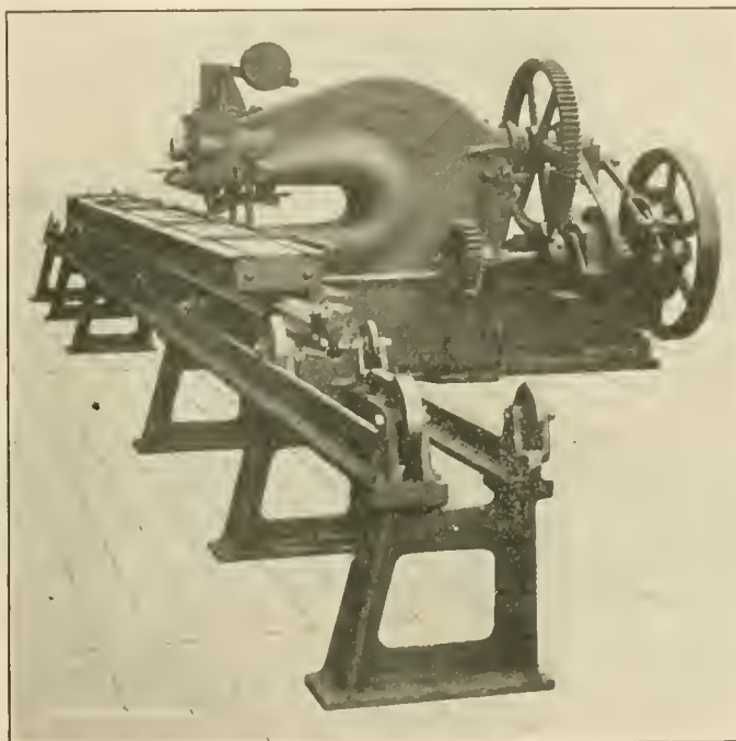
CLEVELAND PUNCH WITH AUTOMATIC SPACING TABLE.
